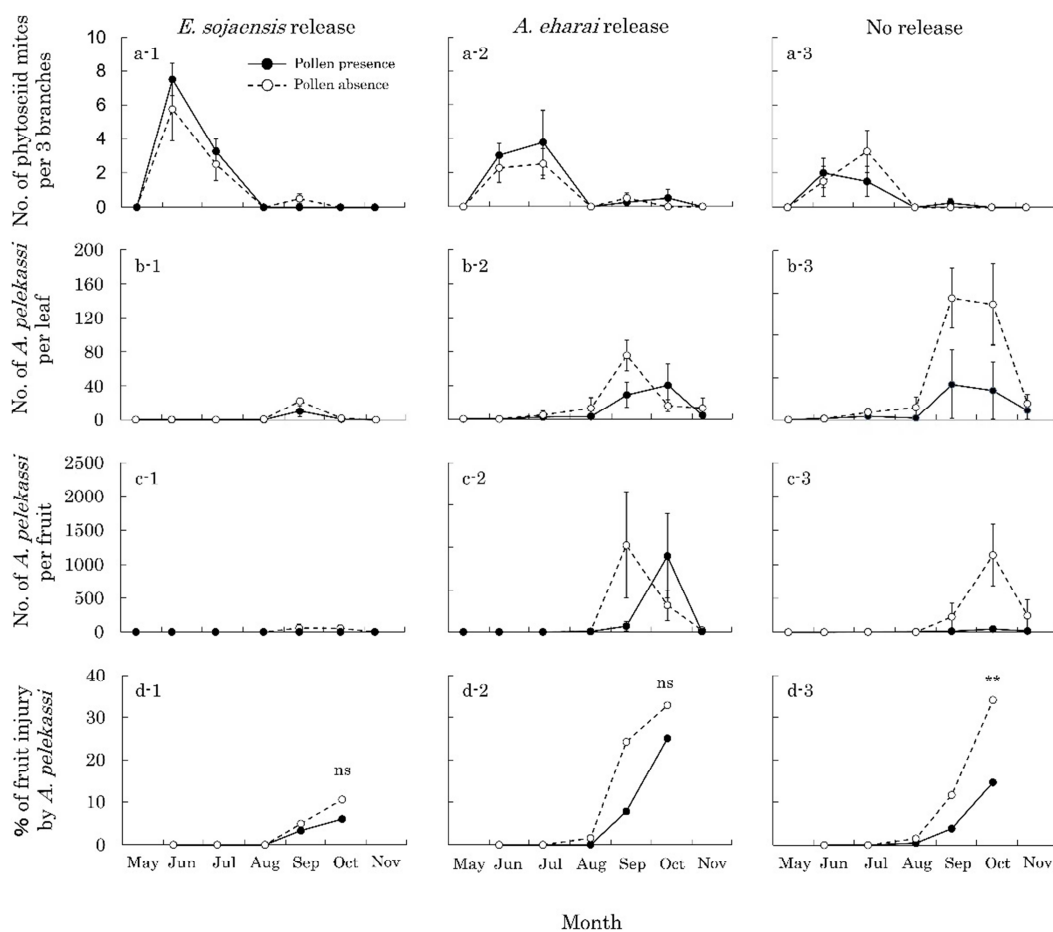
Fig. 3 Seasonal fluctuations in average numbers of (a) phytoseiid mites, (b) A. pelekassi on leaves, (c) A. pelekassi on fruit, and (d) fruit injury on citrus trees in 2016 in three predator release treatments: (1) E. sojaensis release, (2) A. eharai release, and (3) no release. Asterisks indicate a significant difference in fruit injury between treatments with and without pollen in October, according to a chi-squared test weighted by using the Bonferroni correction (** P < 0.01/3 ). 'ns' indicates no significant difference. Error bars indicate SE
